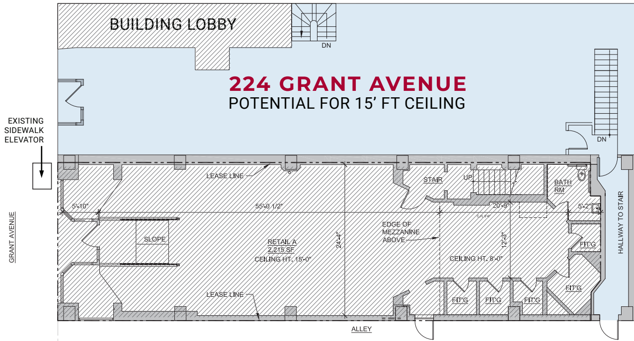
GROUND FLOOR PLAN ±2,175 SF
