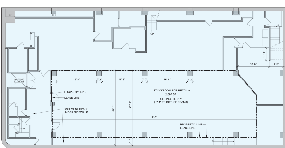
BASEMENT/STOCKROOM PLAN ±4,000 SF
